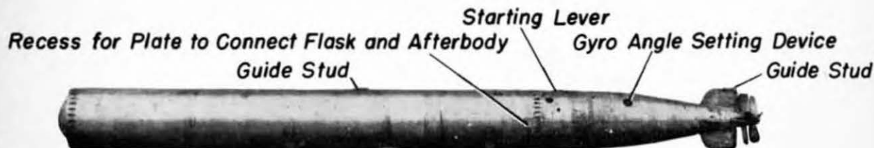
Figure 30—Type 6th year torpedo with warhead removed.
