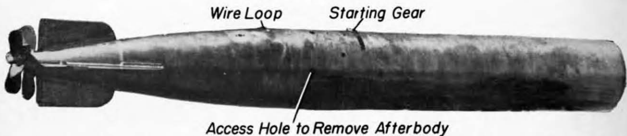
Figure 38—Torpedo type 2 (special) with warhead removed. It is powered by an 8-cylinder radial steam engine.
