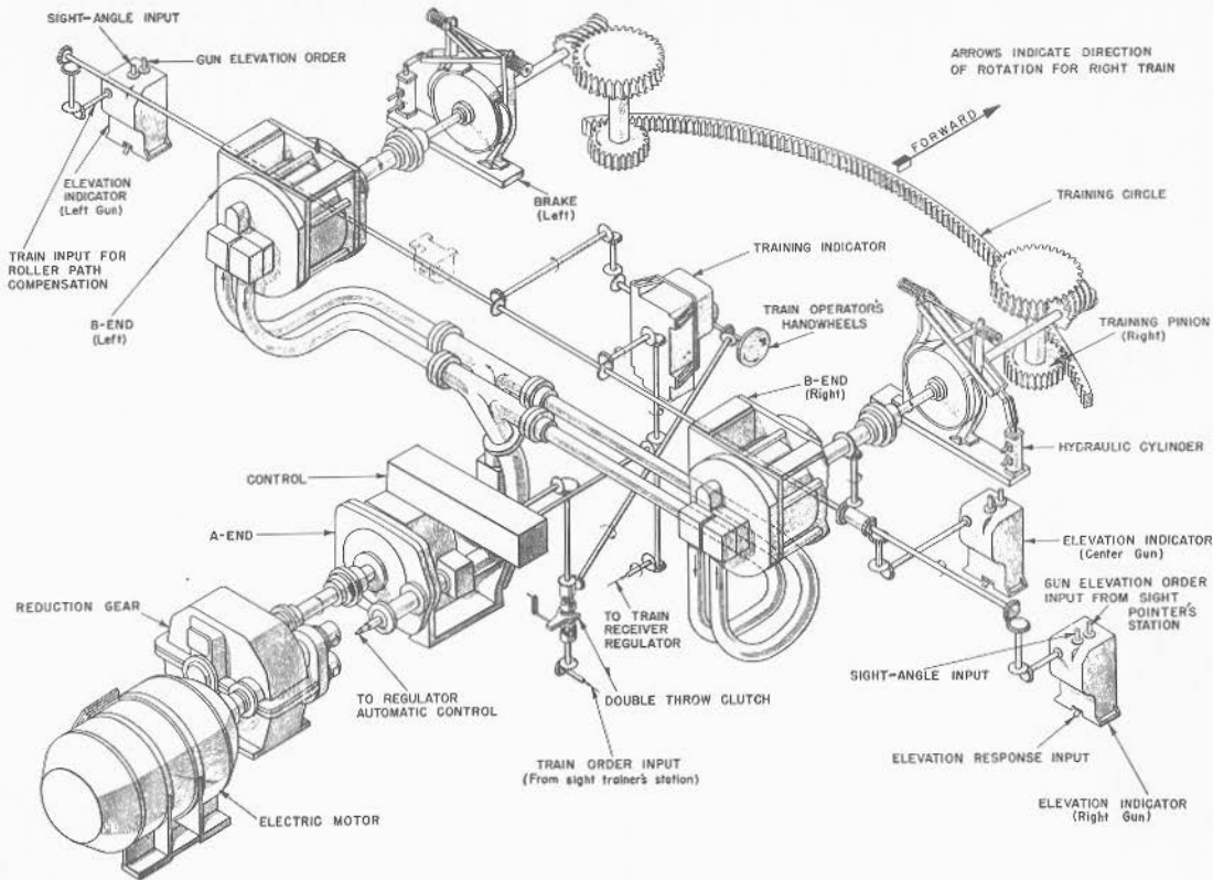
FIGURE 7D2.—Training gear for 16-inch gun.
