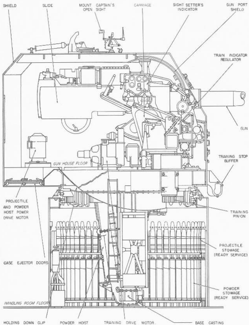
FIGURE 8C2.—5"/51 caliber mount—right side, longitudinal section.
