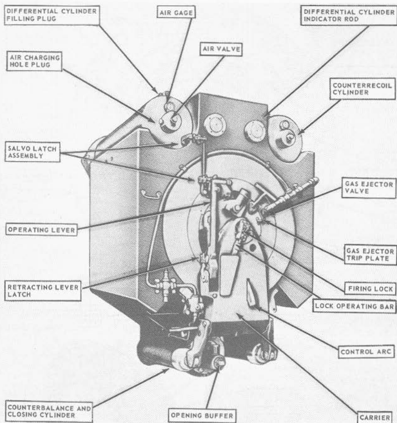
FIGURE 7B2.—16-inch breech mechanism, breech closed.
