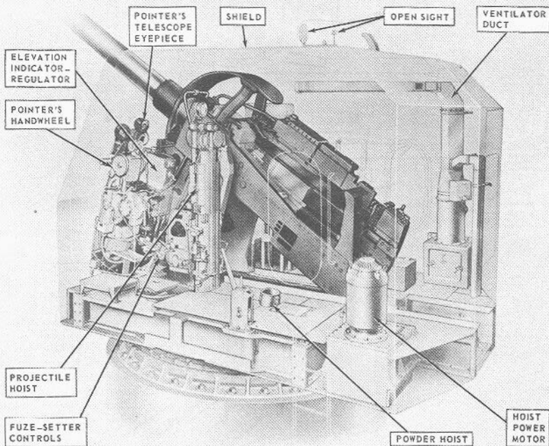
FIGURE 5B1.—Enclosed 5"/54 single mount. (Phantom view.)
