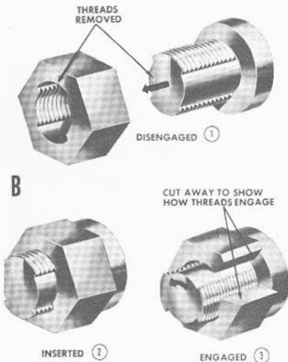
Figure 5B10.—B. Interrupted-screw bolt and nut.
