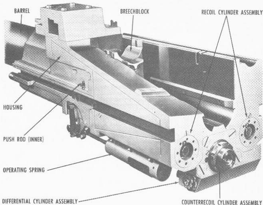
FIGURE 8B1.—5"/38 housing and gun removed from mount.
