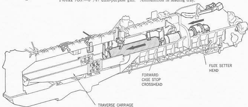
FIGURE 7G10.—6"/47 dual-purpose gun. Ammunition moving aft.
