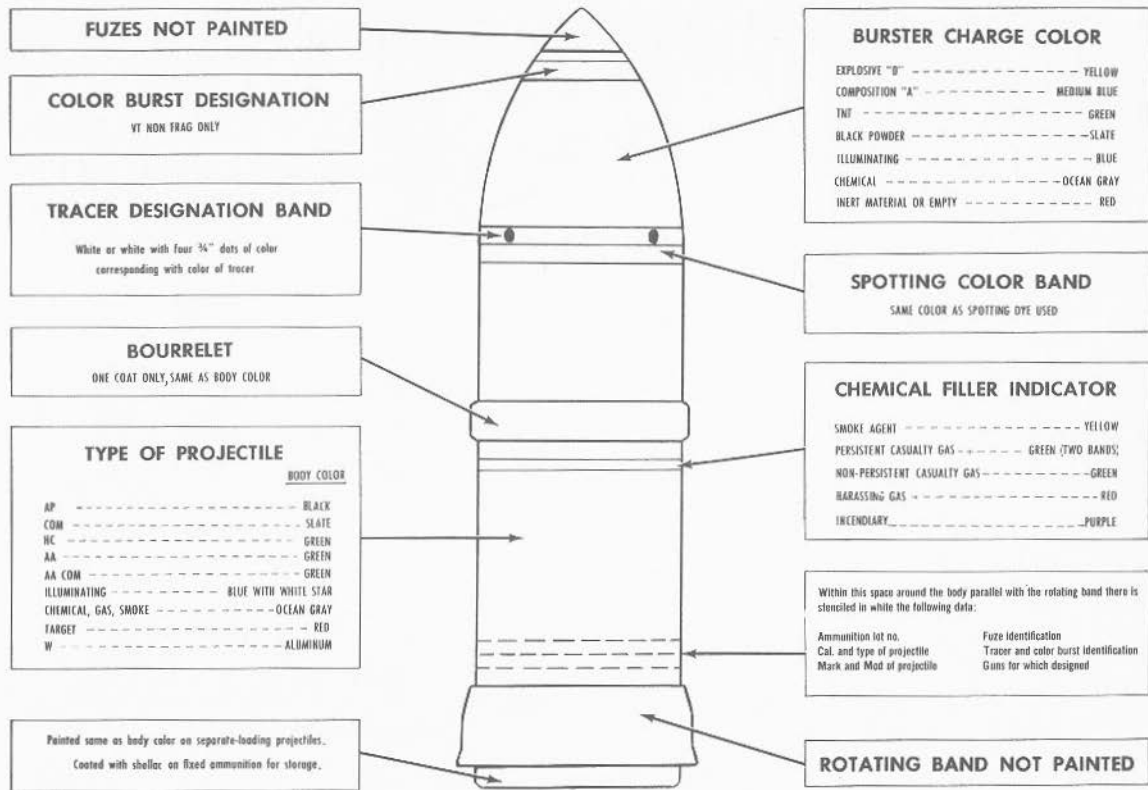
FIGURE 3D5.—Projectile markings.
