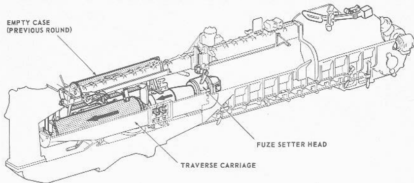
FIGURE 7G11.—6"/47 dual-purpose gun. Ammunition in traverse carriage.
