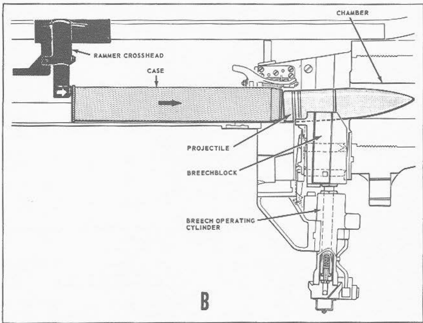
FIGURE 7G15.—6"/47 dual-purpose gun, Ramming.
