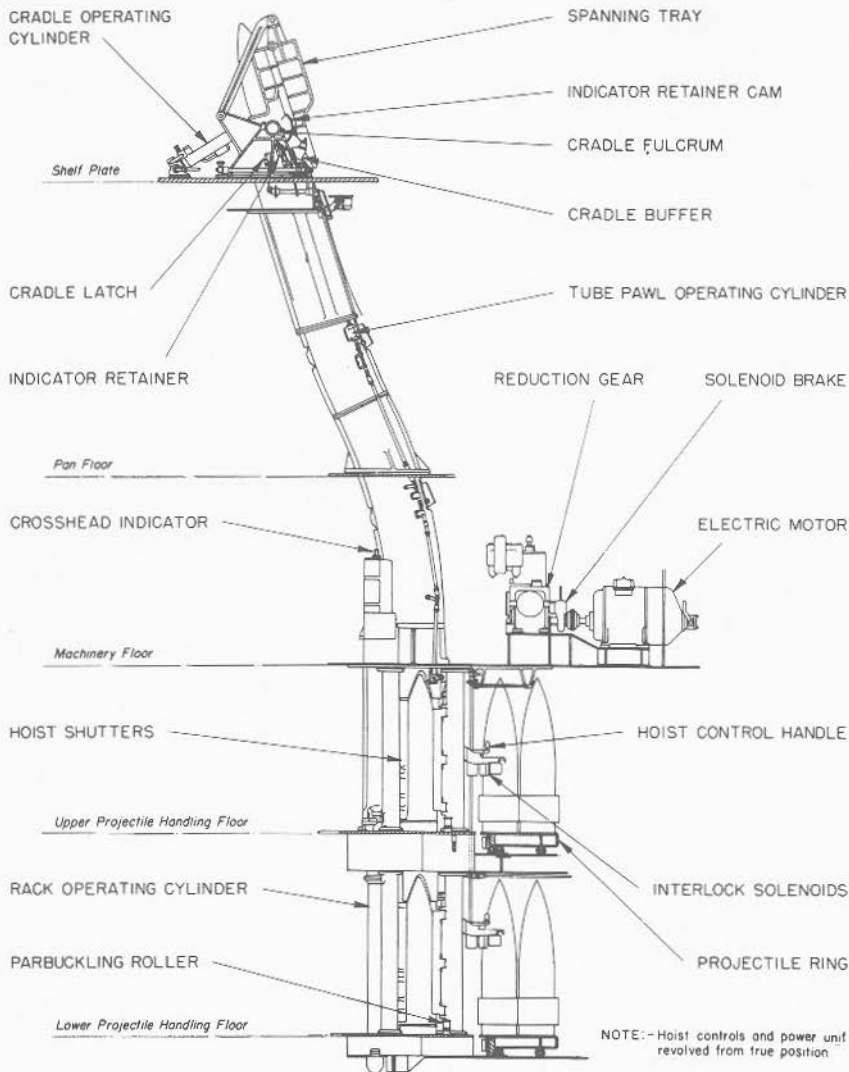
FIGURE 7E3.—16-inch projectile hoist.
