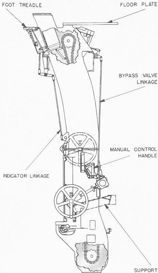
FIGURE 8B21.—Endless-chain powder hoist.
