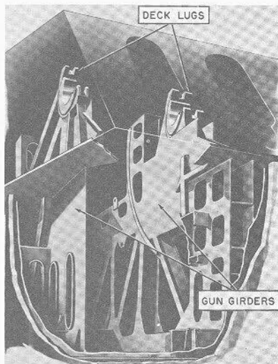
FIGURE 7H4.—8"/55 RF gun and turret. Gun-supporting construction.
