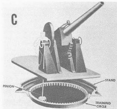
FIGURE 5B3.—C. Principle of training gear.
