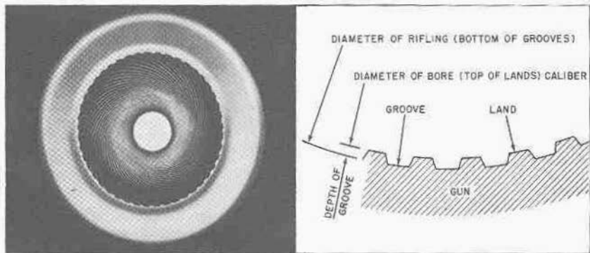
FIGURE 6B5.—Details of gun rifling.
