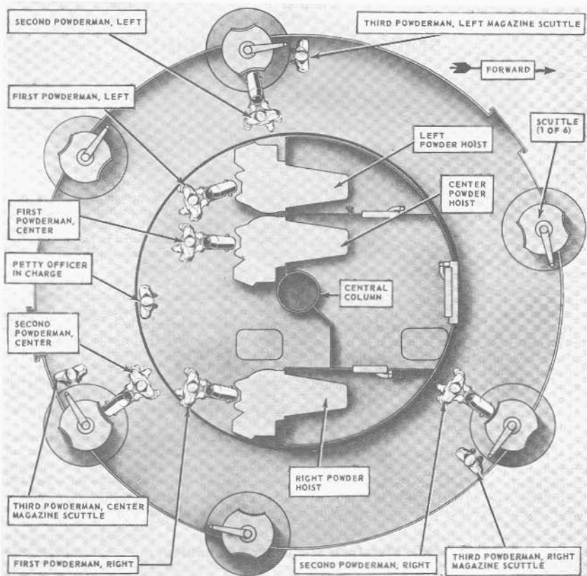
FIGURE 7H29.—8"/55 RF gun and turret. Powder-handling room crew stations.
