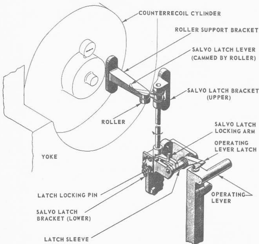
FIGURE 7B4.—Salvo latch for 16-inch gun.
