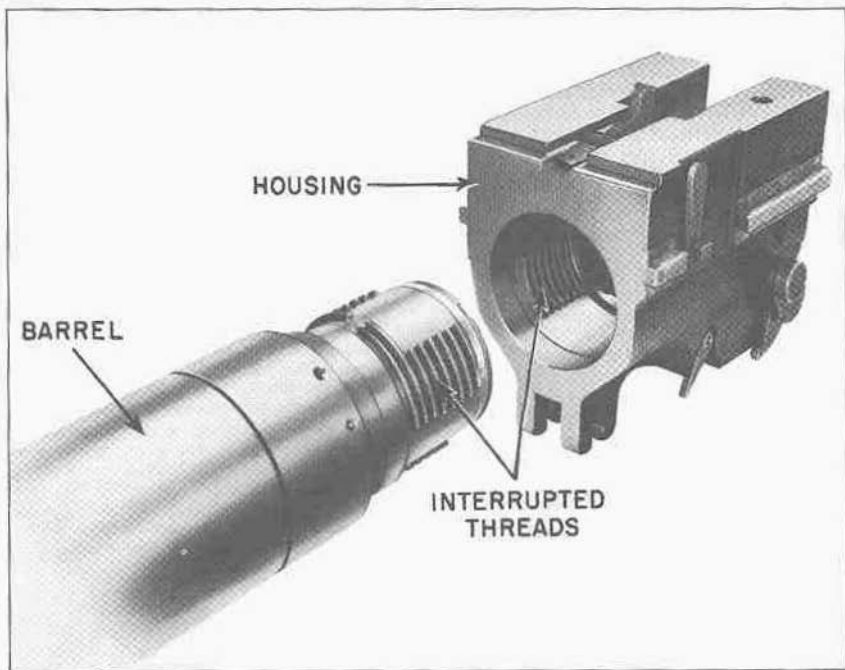
FIGURE 6B6.—Housing-to-barrel joint for case gun.
