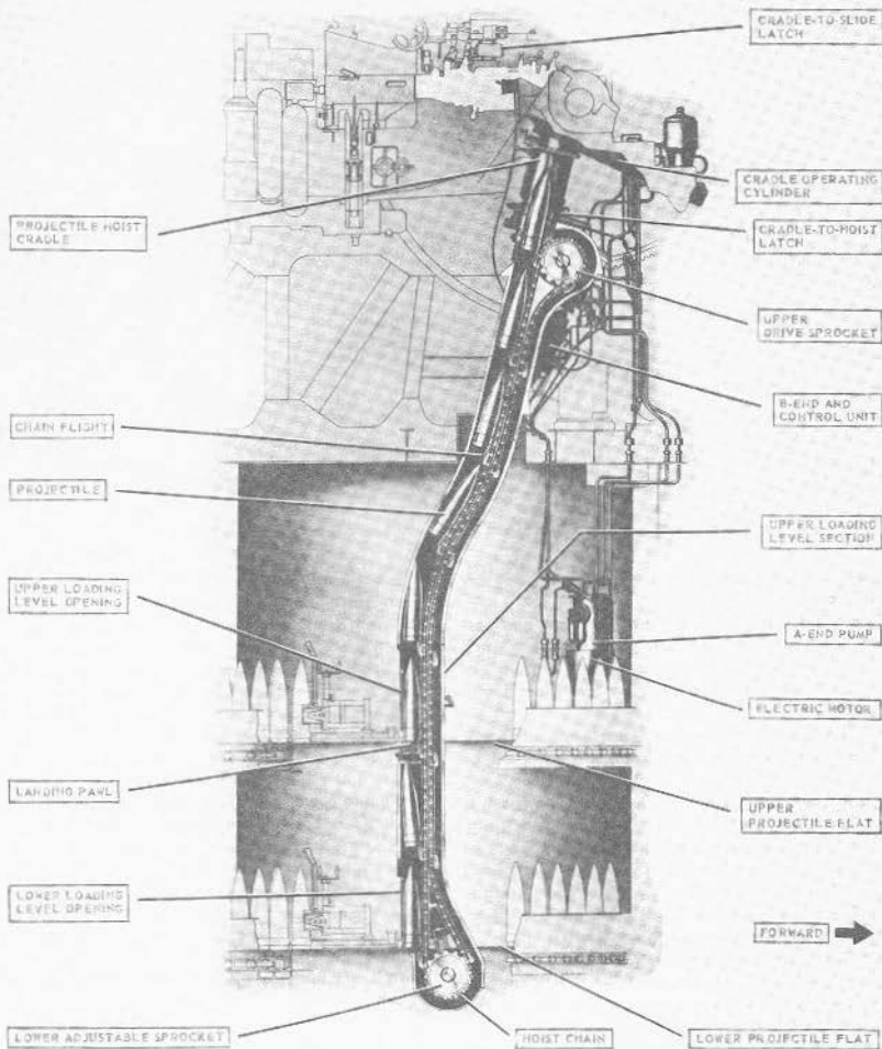
FIGURE 7H9.—8"/55 RF gun and turret. Projectile hoist.
