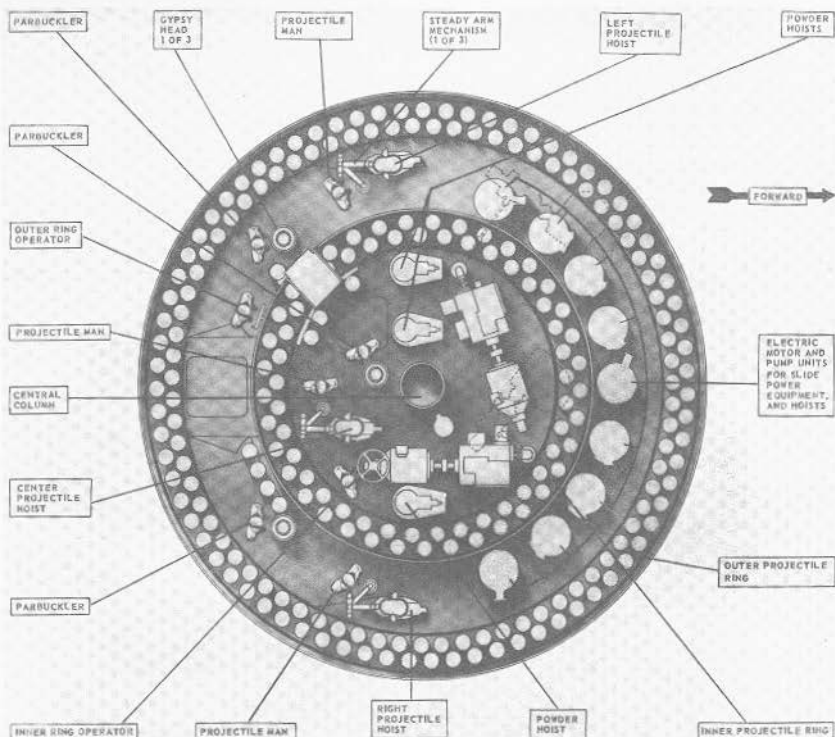
FIGURE 7H28.—8"/55 RF gun and turret. Upper projectile flat crew stations.
