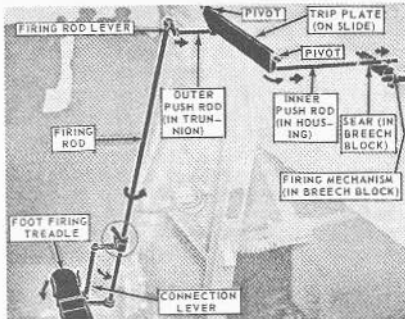
FIGURE 5B17.—5"/38 percussion firing linkage. (Simplified schematic.)
