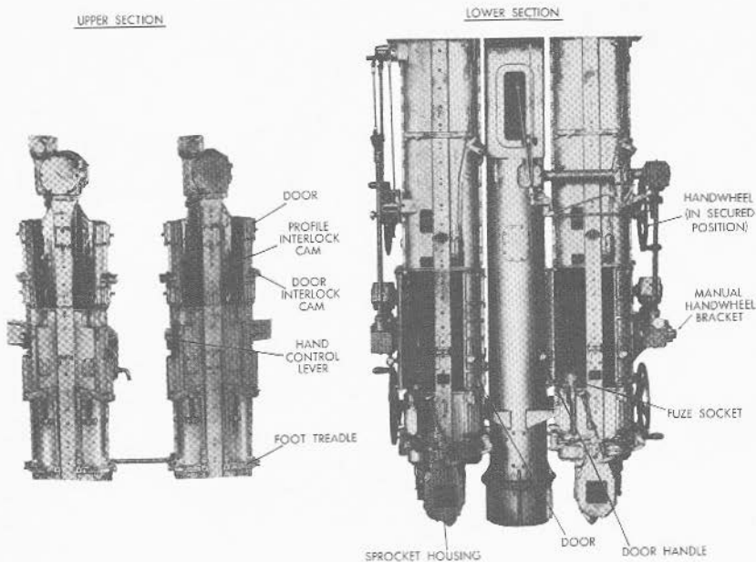
FIGURE 8B17.—5''/38 projectile hoist.
