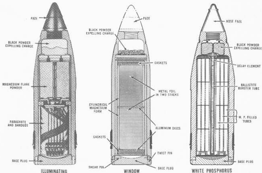
FIGURE 3D4.—Special-purpose projectiles.
