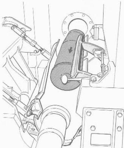
FIGURE 7H23.—8"/55 RF gun and turret. Empty-case tray receives extracted case.
