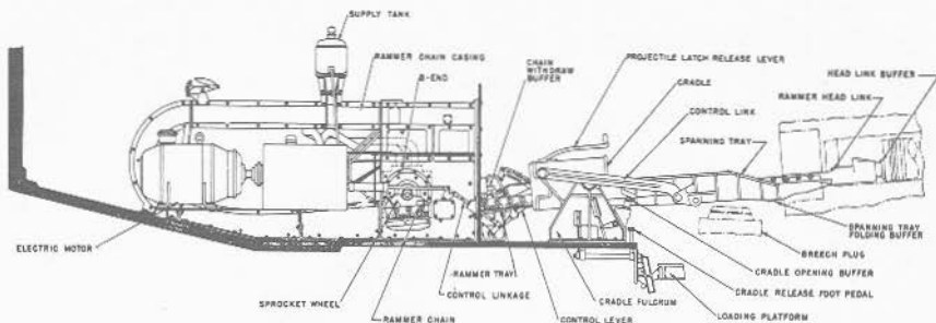
FIGURE 7E6.—Rammer mechanism (16-inch turret).
