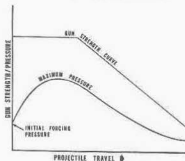
FIGURE 6C3.—Typical gun strength and pressure curves.
