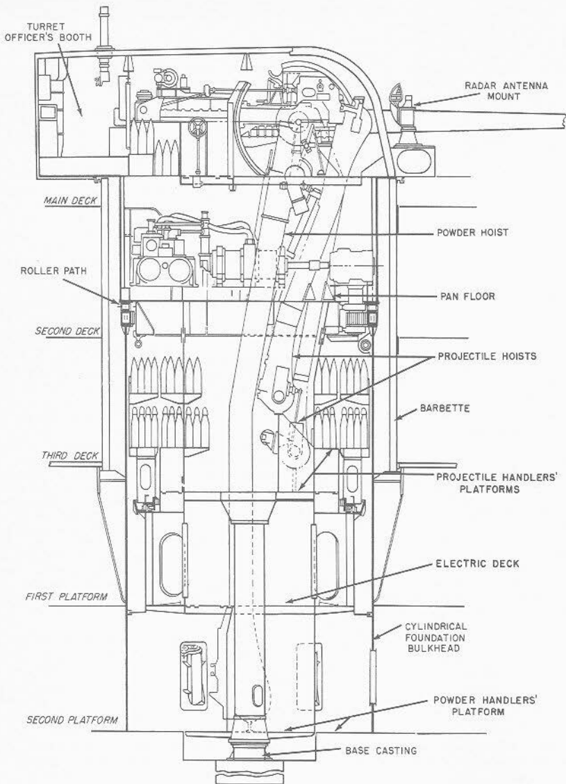
FIGURE 7G1.—Section through 6"/47 dual-purpose two-gun turret.
