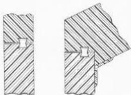
FIGURE 4A2.—Method of keying adjacent plates of Class A armor. Butt joint is shown at left—angle joint at right.
