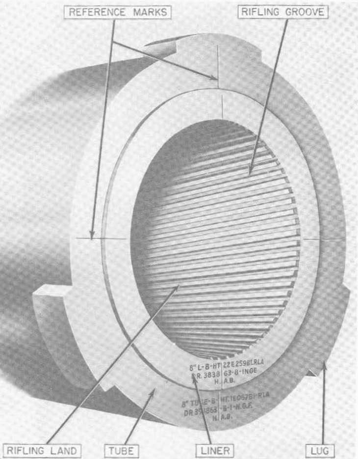
FIGURE 7H3.—8"/55 RF gun and turret. Muzzle, showing rifling and lugs.
