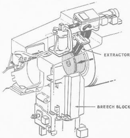
FIGURE 7G17.—6"/47 dual-purpose gun. Case extraction.
