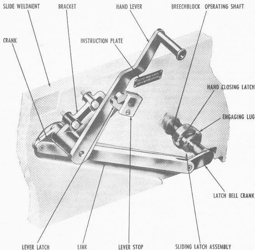
FIGURE 8B10.—5"/38 hand-operating mechanism.
