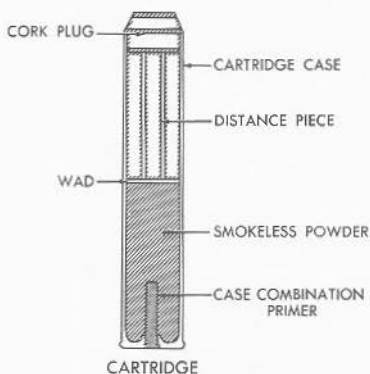
FIGURE 3B4.—5"/38 ammunition (semifixed).
