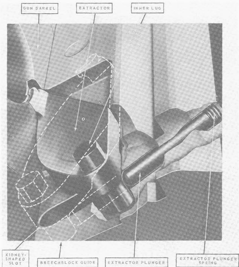
FIGURE 8B6.—Right extractor, 5"/38 gun.
