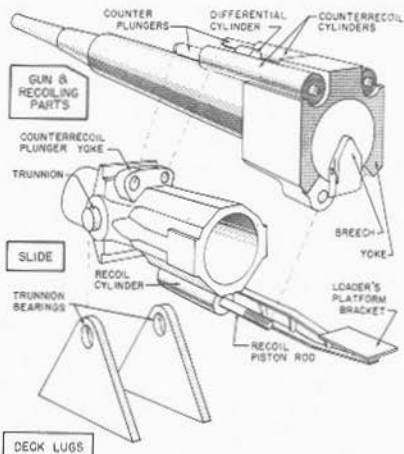
FIGURE 7C1.—16-inch gun assembly. Simplified exploded schematic.
