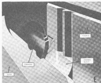
FIGURE 5B6.—E. Breechblock dropping to open position.
