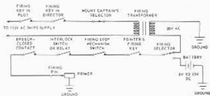
FIGURE 5B19.—Representative electrical firing circuit.
