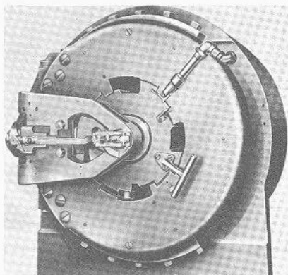
FIGURE 5B11.—Interrupted-screw breech mechanism. Steps in closing.
