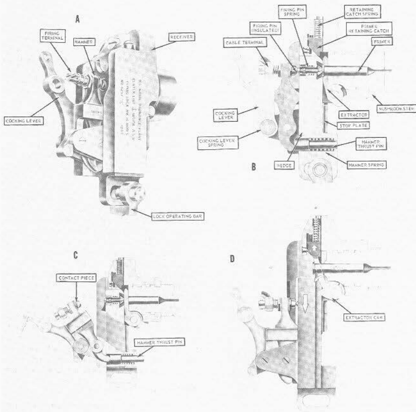
FIGURE 7B5.—Mark 14 firing lock.
