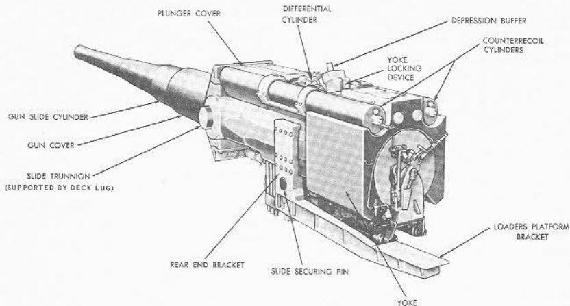
FIGURE 7C2.—16-inch gun assembly, side view (left gun).
