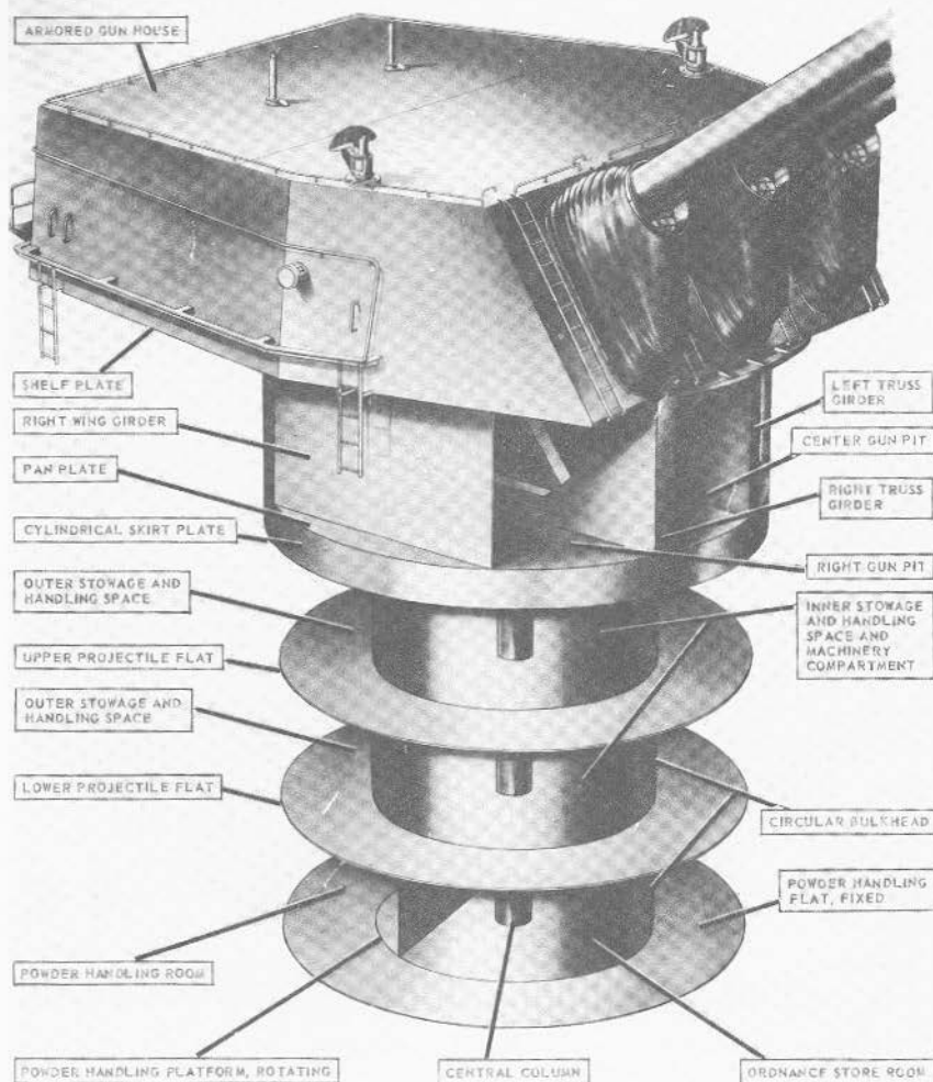
FIGURE 7H2.—8"/55 rapid-fire turret. Rotating structure (simplified).
