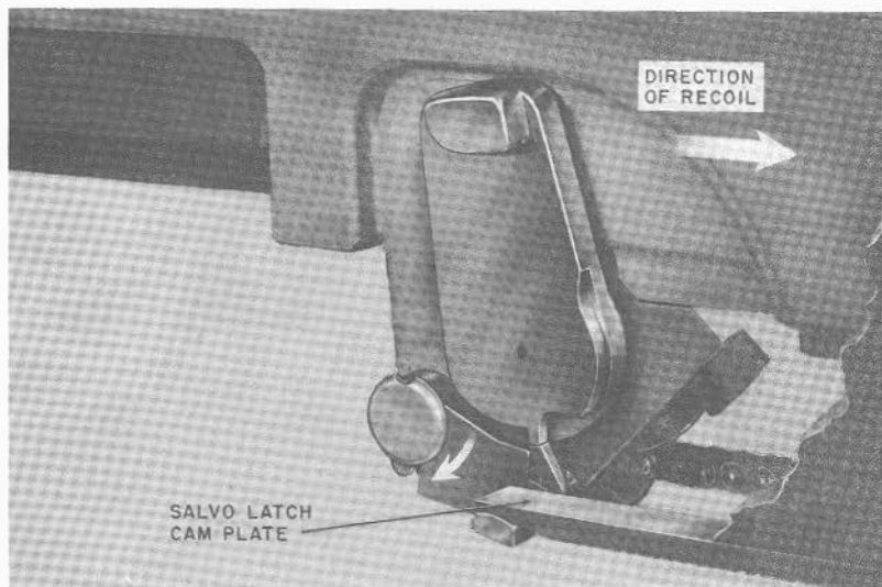
FIGURE 8B8.—5"/38 salvo latch.
