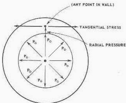
Copyright 1939 by the U. S. Naval Institute FIGURE 6B1.—Forces in a gun cylinder.
