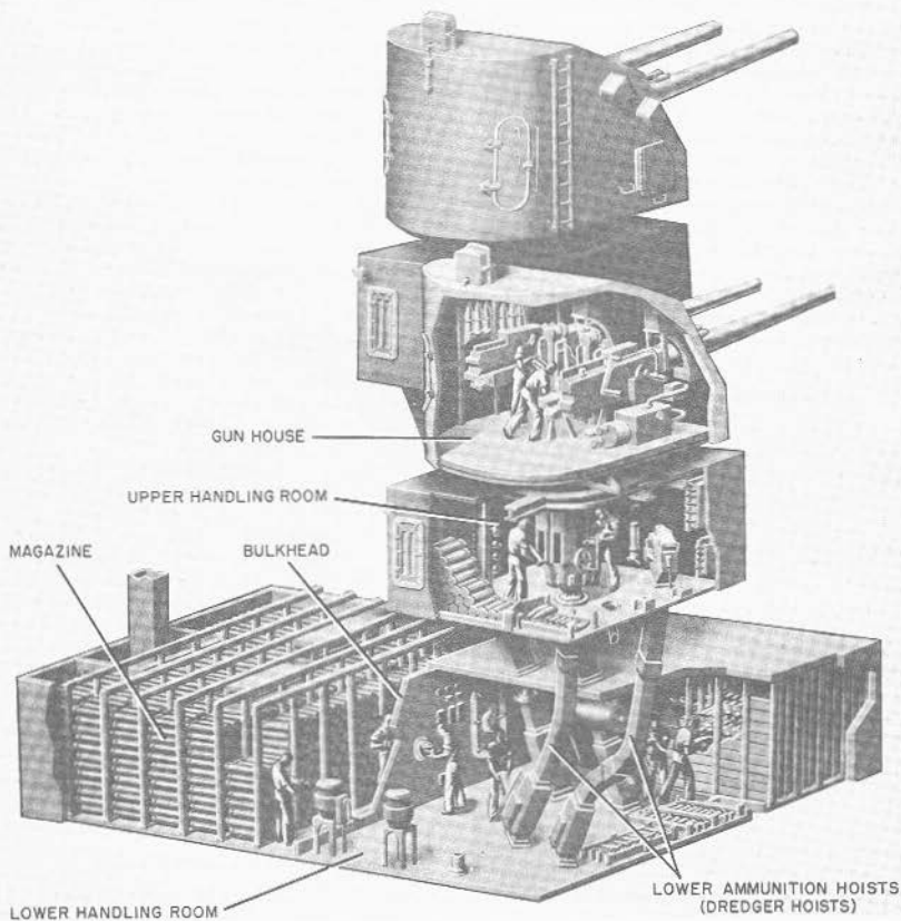
FIGURE 5B29.—Ammunition supply system for 5"/38 twin mount.
