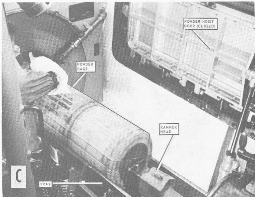
FIGURE 7E5.—(Continued.) C. Loading the powder.
