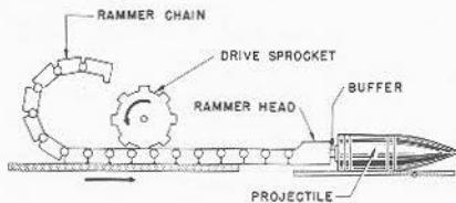
FIGURE 5B28.—Principle of chain-type rammer.
