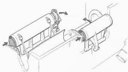
FIGURE 7H15.—8"/55 RF gun and turret. Trays moving toward ramming position.
