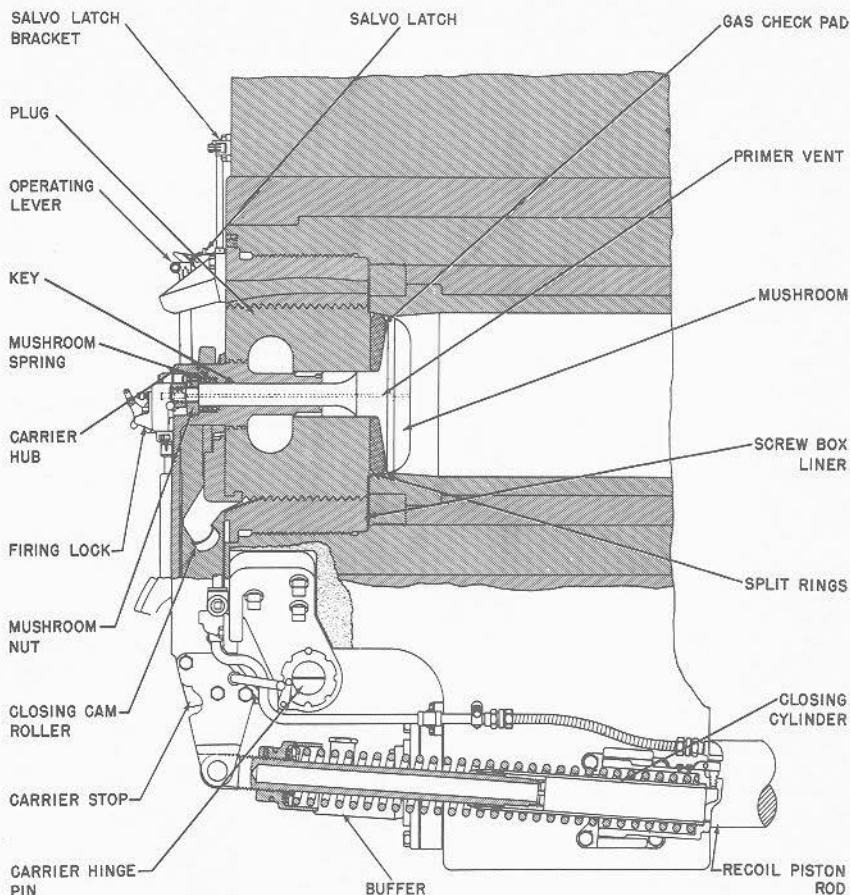
FIGURE 7B3.—Breech plug and carrier.
