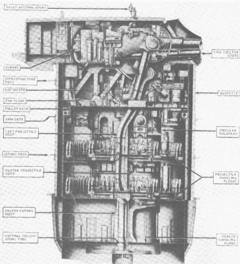
FIGURE 7H1.—8"/55 rapid-fire turret. Cross section.
