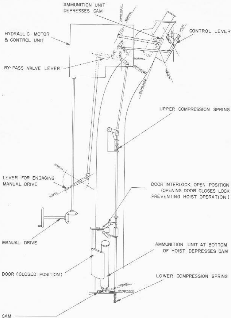
FIGURE 8B22.—5 1/8 caliber powder hoist, hydraulic system control.
