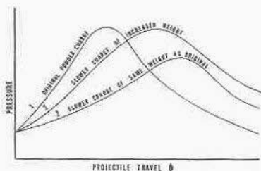
FIGURE 6C5.—Typical gun pressure curves showing methods of obtaining increased muzzle velocity in a gun without increasing maximum pressure.
