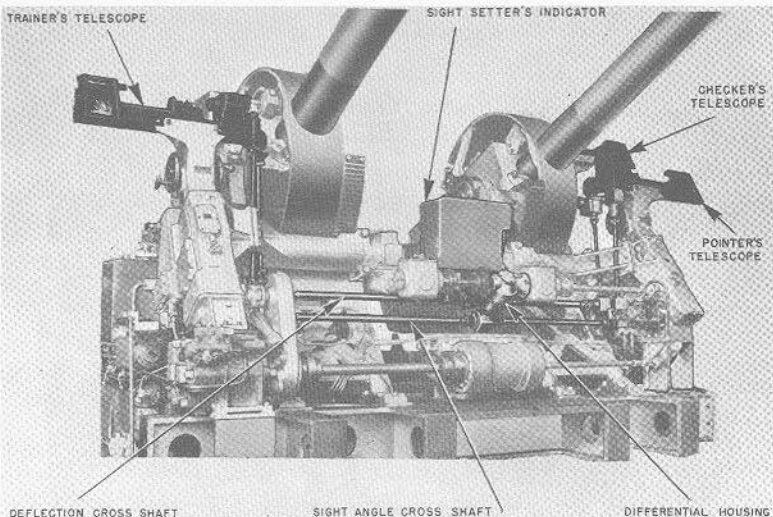
FIGURE 8B23.—Sights in 5"/38 twin mount.
