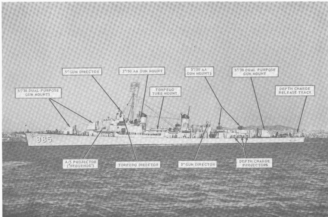
FIGURE 1B2.—Arrangement of weapons on a destroyer.
