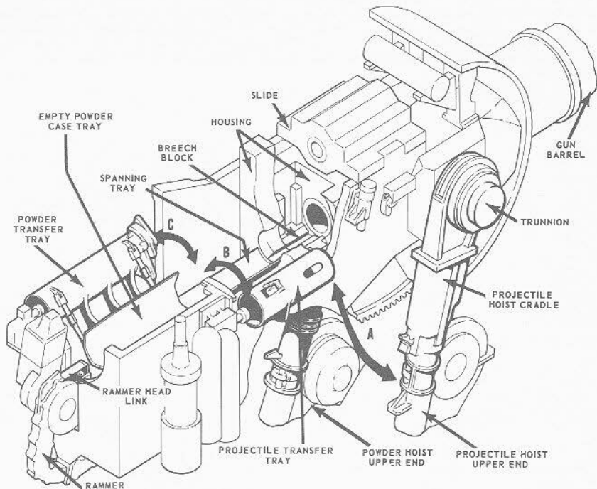
FIGURE 7H11.—8"/55 RF gun and turret. Loading equipment.
