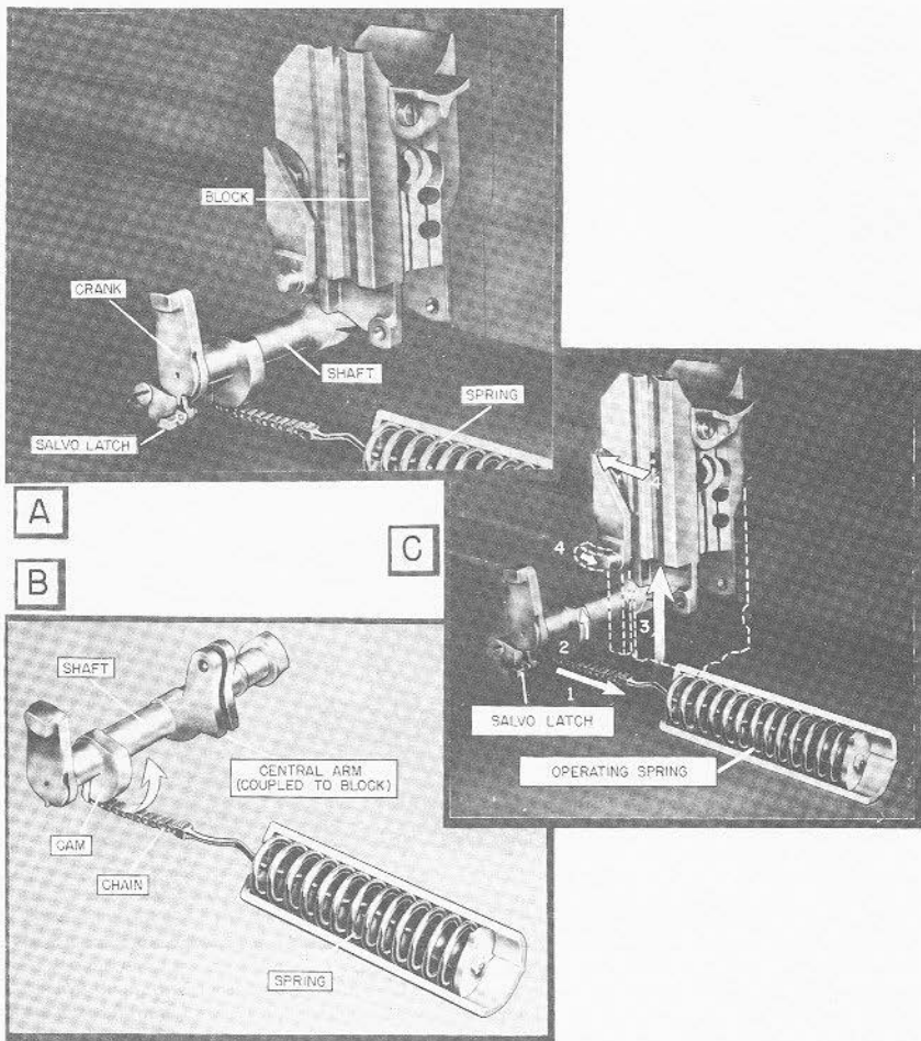
FIGURE 8B7.—Parts and functions of 5 1/8 inch/38 breech mechanism.
