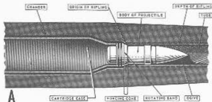
FIGURE 5B9.—A. Cross section of gun chamber (fixed ammunition).
