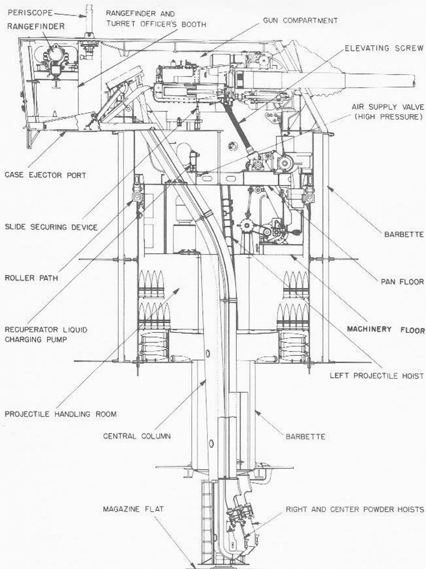
FIGURE 7F1.—Section through 6"/47 triple gun turret.
