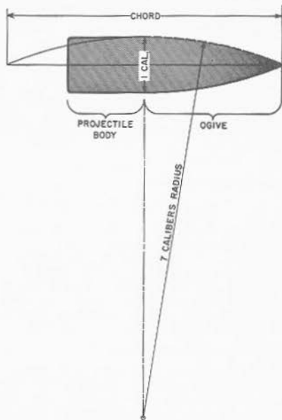
FIGURE 3D1.—Ogive characteristics.
