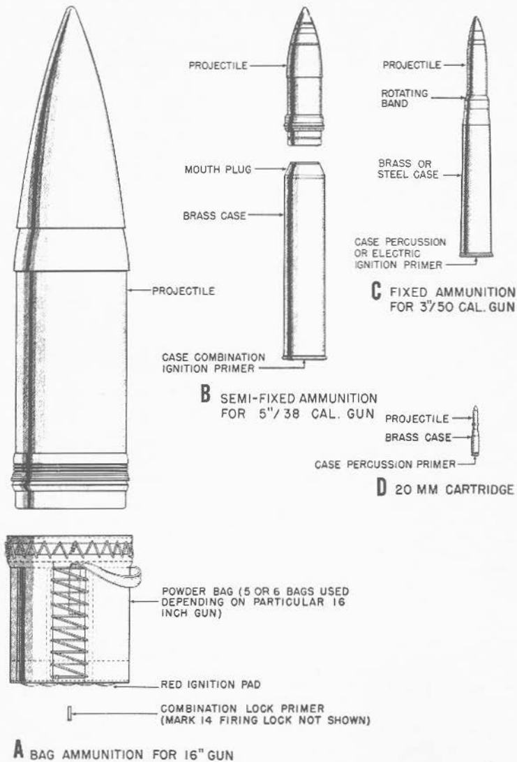
FIGURE 3B1.—Typical gun ammunition.
