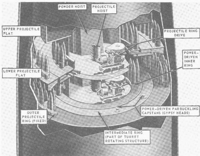
FIGURE 7E1.—Projectile flats in 16-inch turret.
