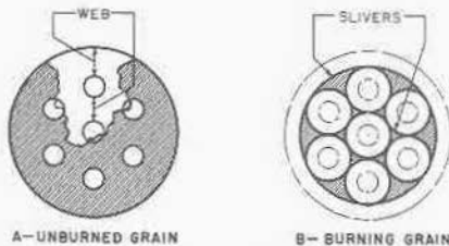
FIGURE 6C1.—Burning surface of perforated powders.
