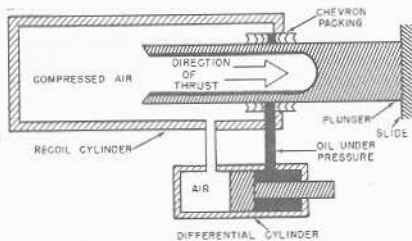
FIGURE 5B23.—Hydro-pneumatic counterrecoil system. (Simplified schematic.)
