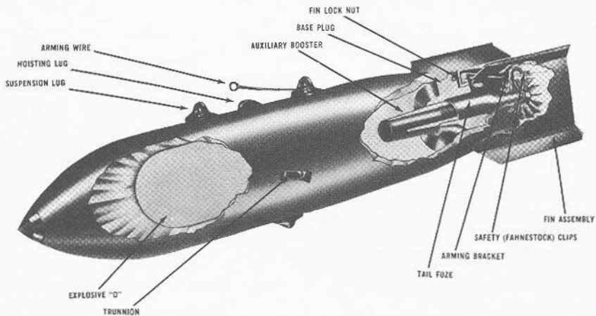
FIGURE 3F2.—An armor-piercing bomb assembled for loading.
