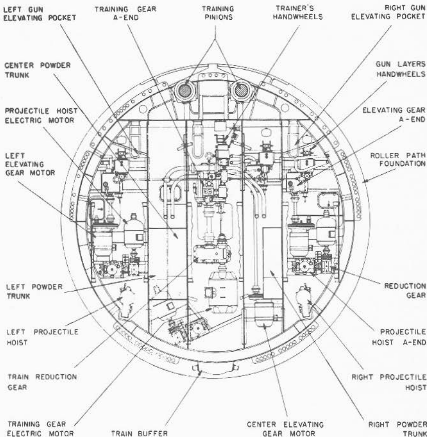
FIGURE 7A4.—Machinery floor, plan view, 16"/50 caliber gun turret.
