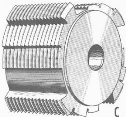
FIGURE 5B10.—C. Stepped-thread plug (Welin type).
