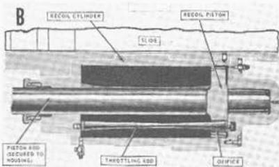
FIGURE 5B22.—Hydraulic recoil brakes. A. Throttling-groove type. B. Throttling-rod type.
