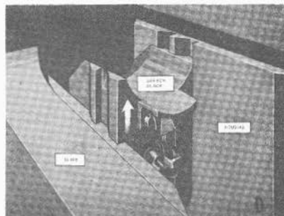
FIGURE 5B6.—D. Breechblock rising to closed position.
