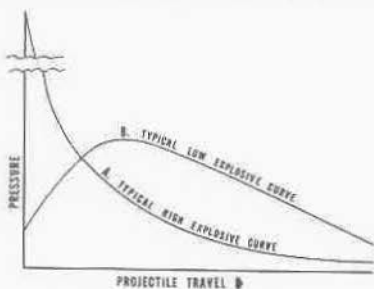
FIGURE 6C2.—Gun pressure curves.
