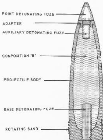
FIGURE 3D3.—6"/47-caliber high-capacity projectile.
