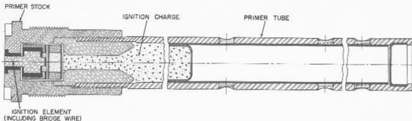
FIGURE 3C2.—Case electric primer.
