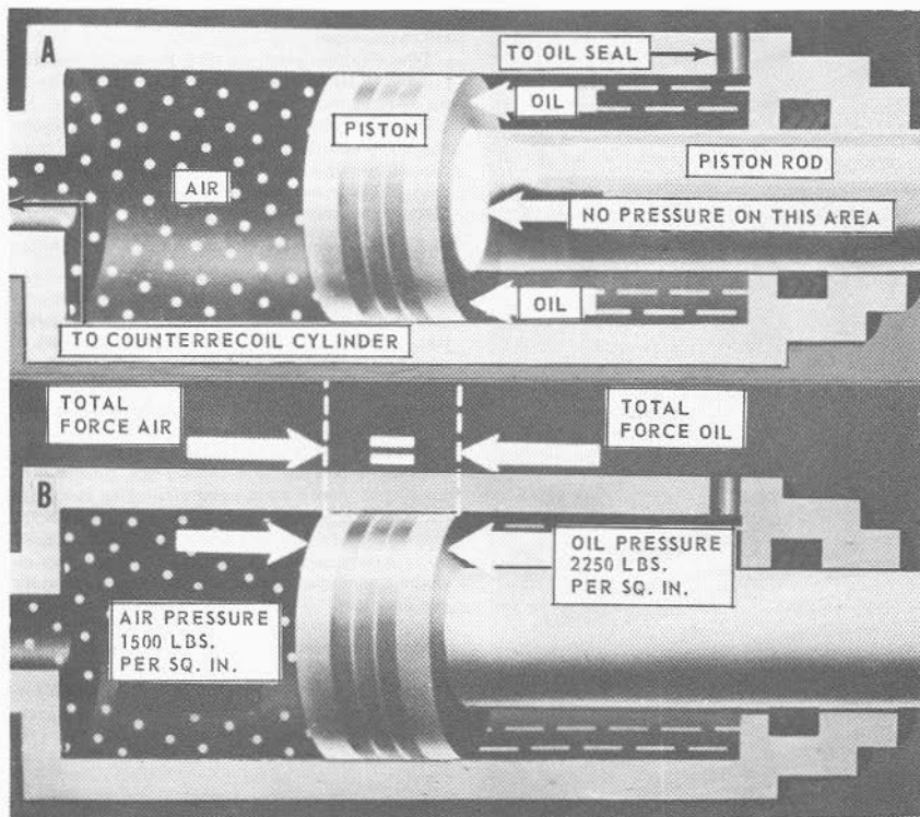
FIGURE 5B25.—Hydropneumatic counterrecoil system. Principle of differential cylinder.
