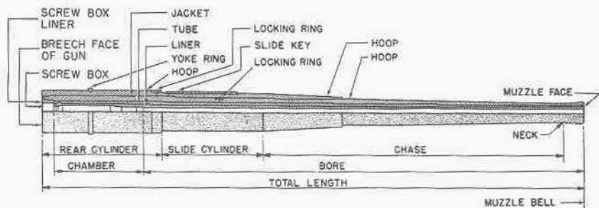
FIGURE 6B3—Built-up major caliber gun. (Cross section.)
