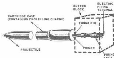
FIGURE 5B16.—Firing mechanism for sliding-wedge breech mechanism.
