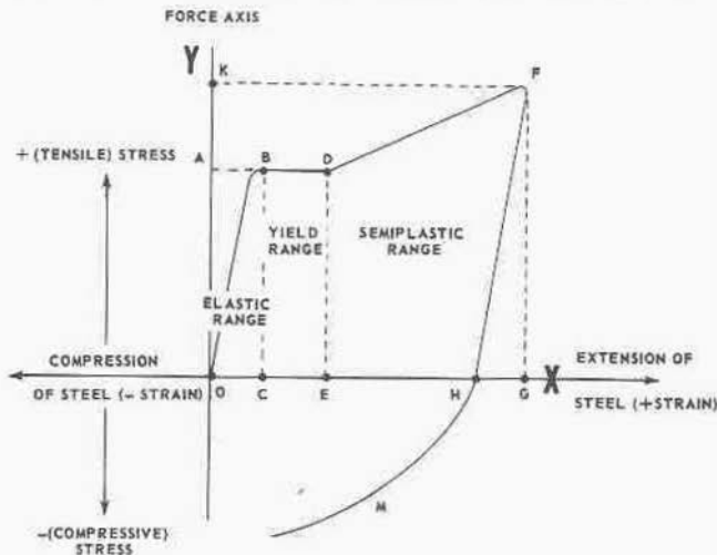
FIGURE 6B2.—Stress and strain in a gun cylinder.
