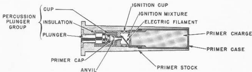
FIGURE 3C4.—Lock combination primer.
