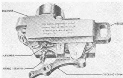
FIGURE 5B18.—Mark 14 firing lock (for bag guns).
