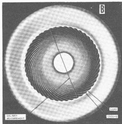
FIGURE 5B9.—B. Rifled bore (viewed head-on).
