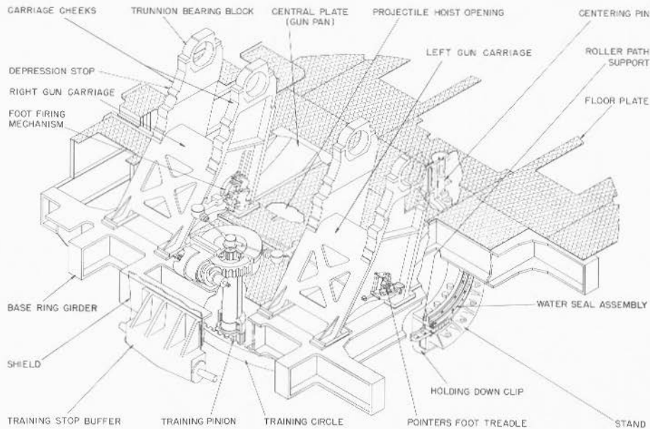
FIGURE 8B15.—5 1 / 8 twin-mount stand and carriage.
