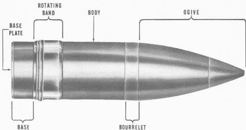
FIGURE 3D2.—Main parts of projectile.
