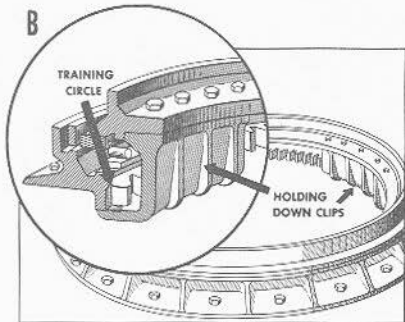
FIGURE 5B3.—B. Training circle and holding-down clips.
