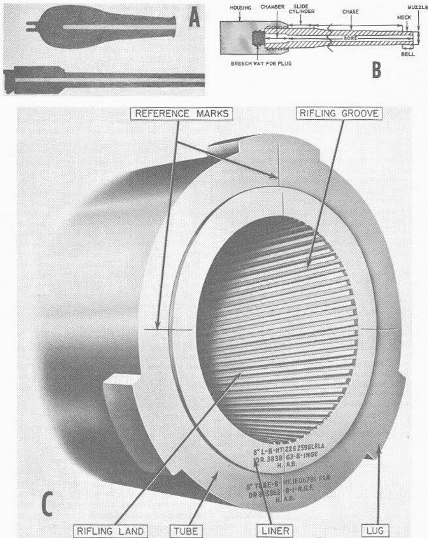
FIGURE 5B7.—The gun barrel. A. Old and new gun barrel profiles. B. Main parts of the barrel. C. Muzzle end of 8-inch turret gun, showing the rifling and the liner.
