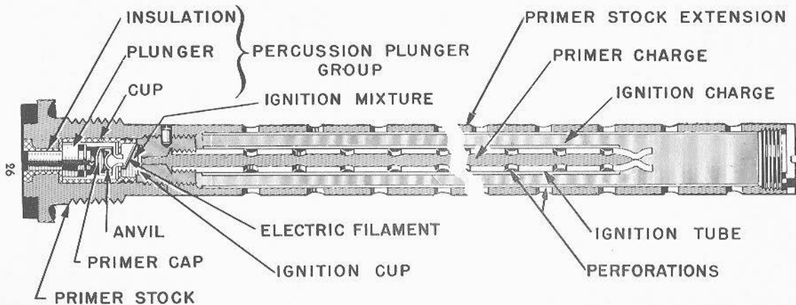
FIGURE 3C3.—Case combination primer.
