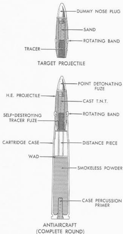
FIGURE 3B3.—40-mm ammunition (fixed).
