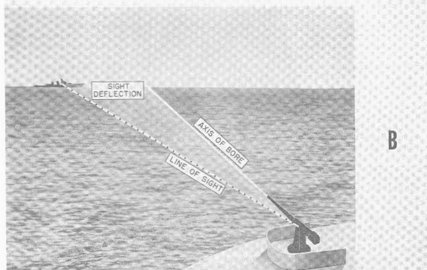
FIGURE 5B33.—Sight angle (A) and sight deflection (B).
