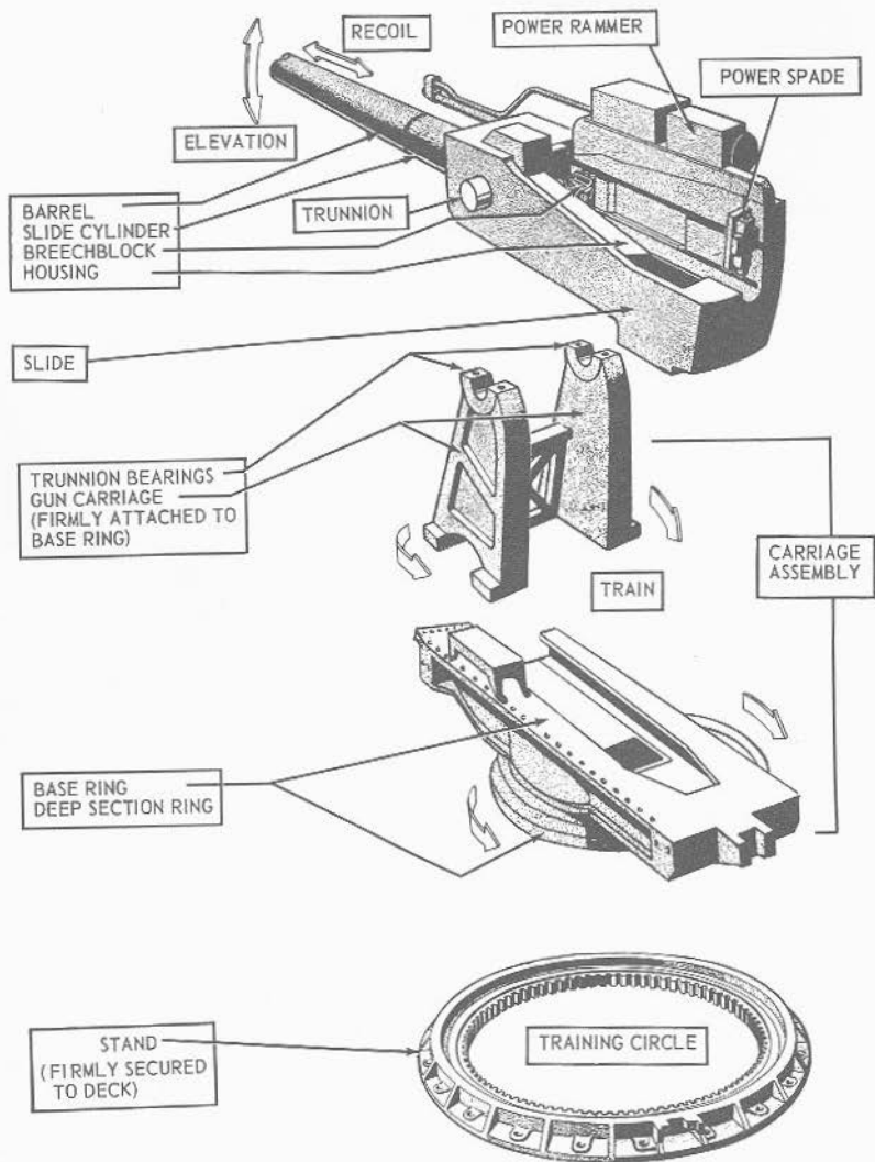
FIGURE 5B2.— Main assemblies of a 3-inch mount. (Exploded view.)
