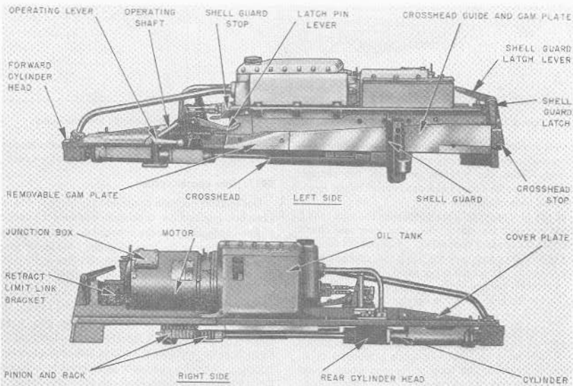
FIGURE 8B12.—5"/38 rammer, assembled arrangement.
