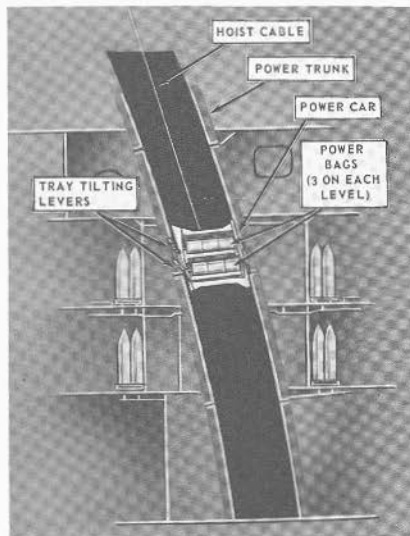
FIGURE 7E4.—Powder car and trunk for 16-inch turret.
