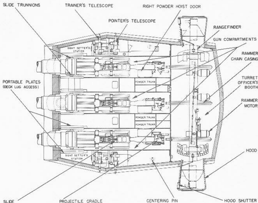
FIGURE 7A2.—Plan view of turret gun house.
