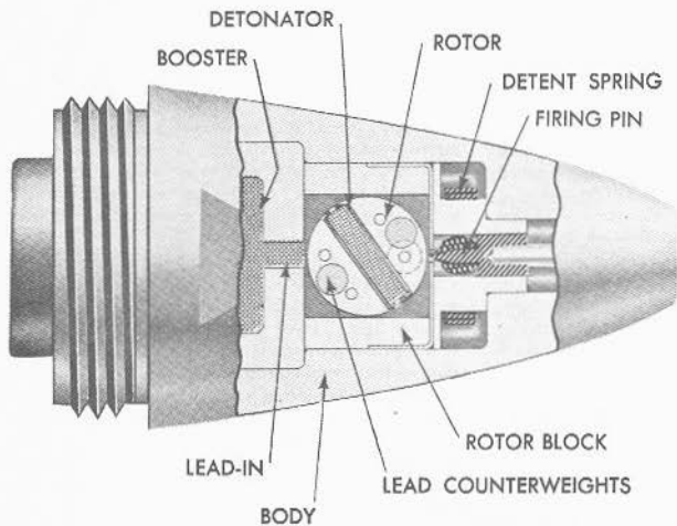
FIGURE 3E2.—Two views of point detonating fuze—unarmed.
