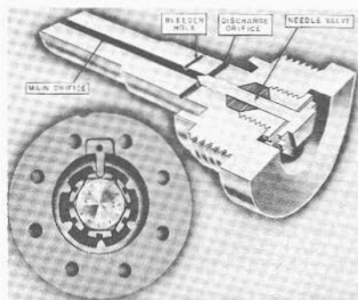
FIGURE 5B26.—Counterrecoil buffer functioning.
