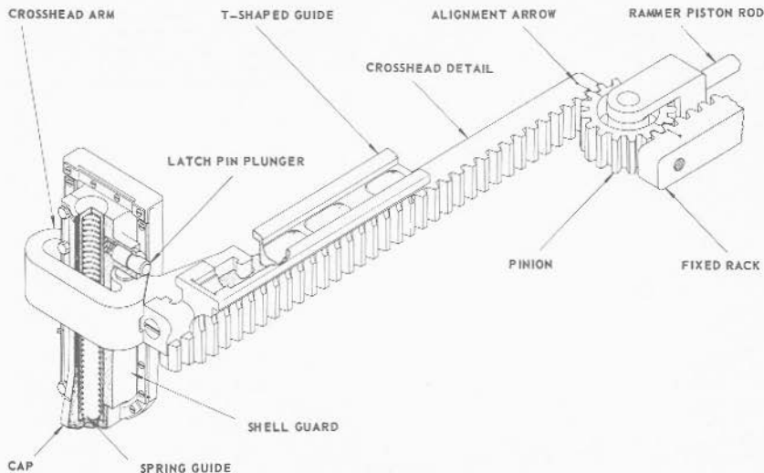
FIGURE 8B13.—5"/38 rammer pinion and rack arrangement.
