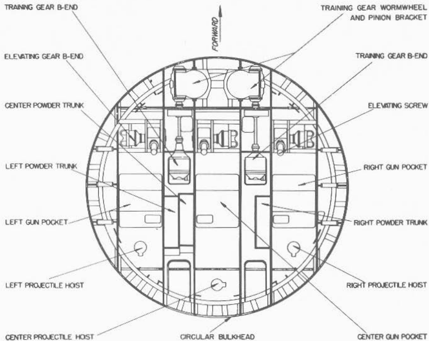
FIGURE 7A3.—Pan floor, plan view, 16"/50 gun turret.
