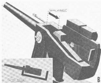
FIGURE 5B6.—B. Recoil movement.
