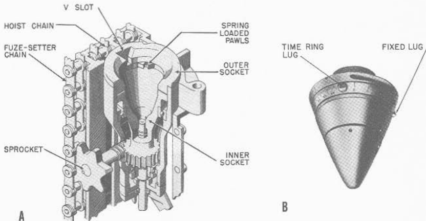
FIGURE 8B20.—Fuze-setting mechanism, 5 1 / 8 caliber gun. A. Projectile flight. B. Fuze.
