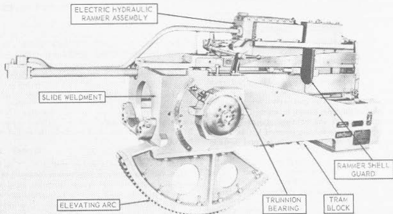
FIGURE 8B2.—5"/38 slide (single mount type).
