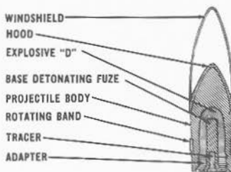
FIGURE 4B2.—Common projectile.
