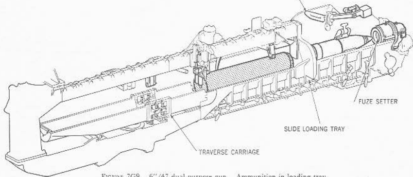
FIGURE 7G9.—6"/47 dual-purpose gun. Ammunition in loading tray.
