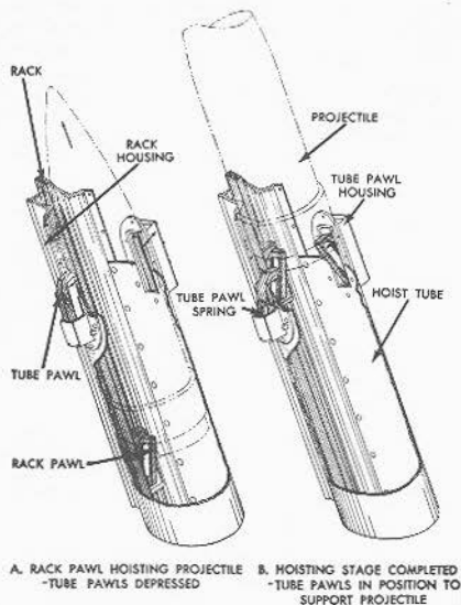
FIGURE 5B32.—Principle of pawl-type hoist.
