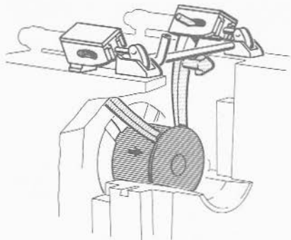
FIGURE 7H22.—8"/55 RF gun and turret. Extractor action.
