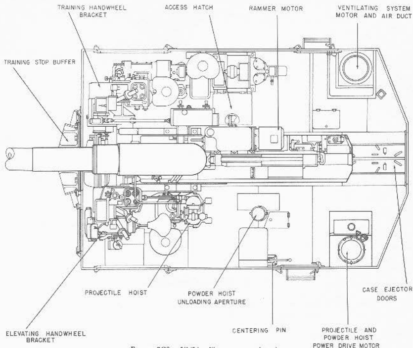
FIGURE 8C3.—5"/54 caliber mount—plan view.
