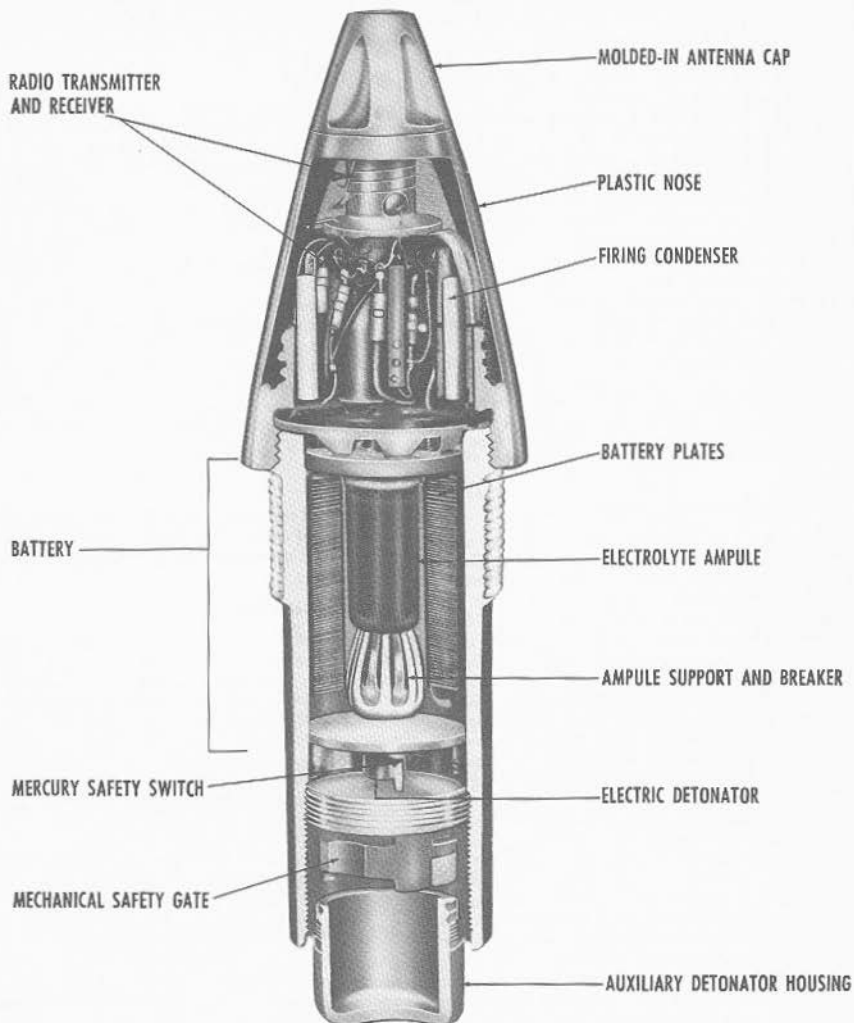
FIGURE 3E3.—Typical VT fuze.
