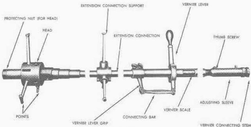
FIGURE 6D1.—The star gage.
