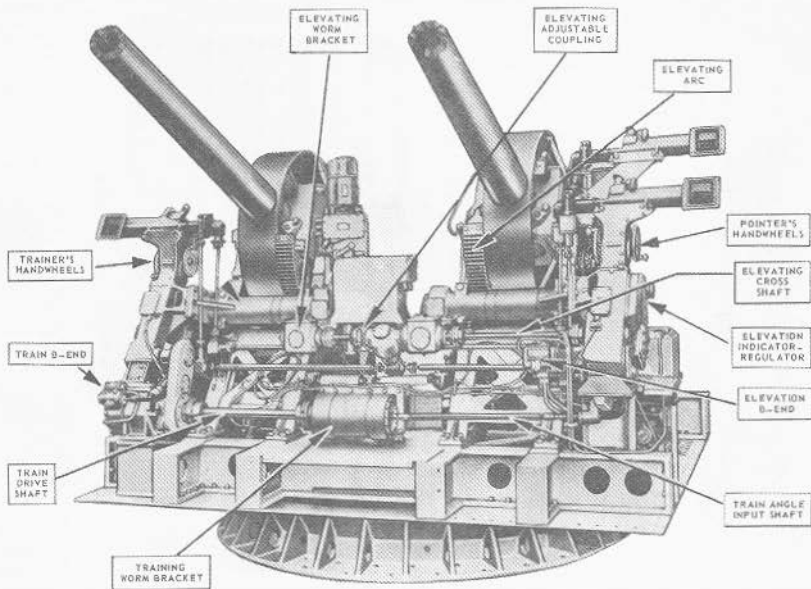
FIGURE 8B16.—5"/38 twin-mount elevating and training gear.
