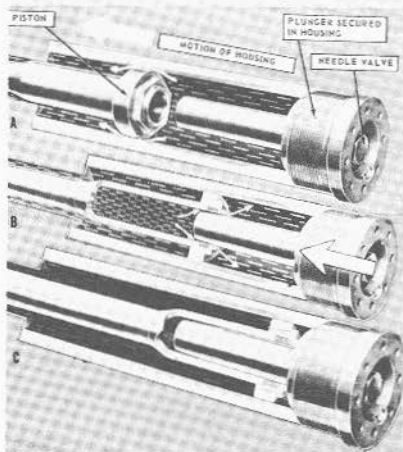
FIGURE 5B26.—(Continued.) Needle valve control.
