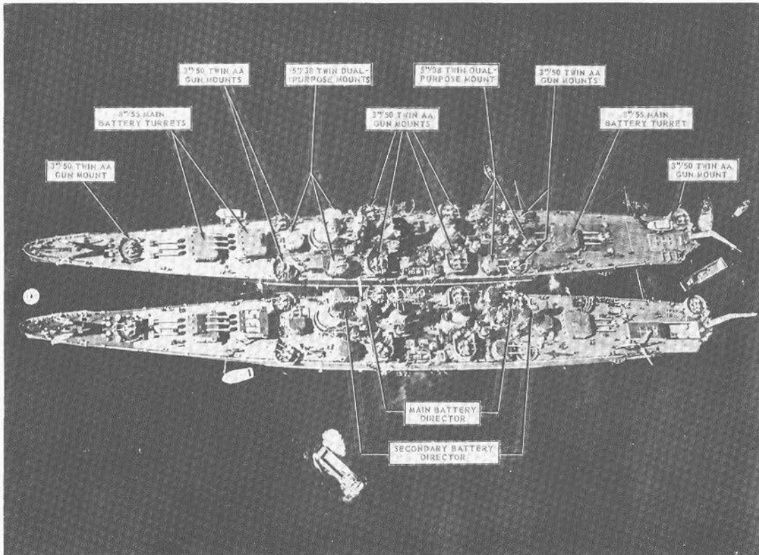
FIGURE 1B1.—Armament arrangement on a cruiser.
