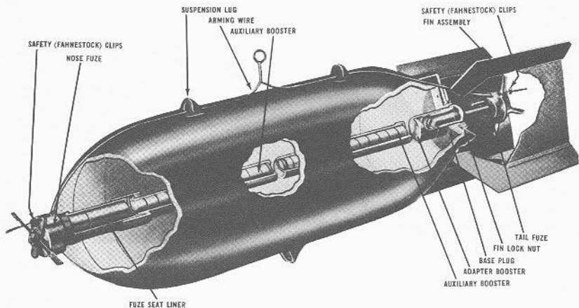
FIGURE 3F3.—A general-purpose bomb assembled for loading.
