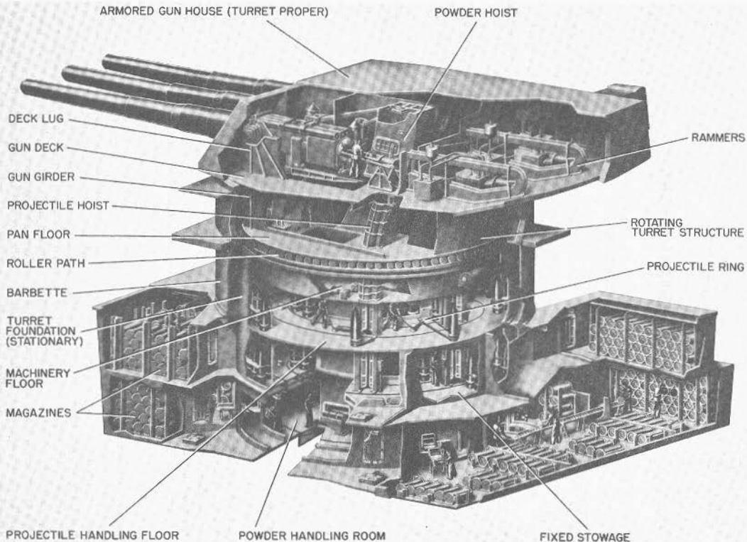
FIGURE 7A1.—Cutaway view of a modern turret (16-inch).
