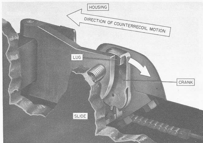
FIGURE 8B9.—5"/38 operating-shaft cam plate.
