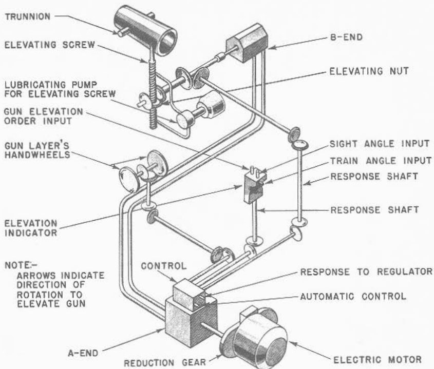
FIGURE 7D1.—Elevating gear for 16-inch gun.
