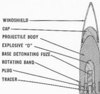
FIGURE 4B1.—Armor-piercing projectile.
