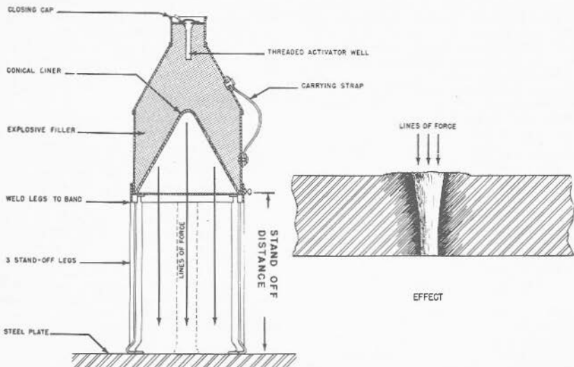
FIGURE 3A1.—Shaped charge and its effect.
